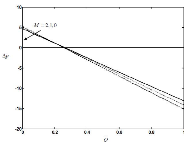
Fig. 14 The variation of the pressure rise \Delta p with \bar{Q} for different values of M with n = 0.5 , \beta = 0.1 , m = 0.2 , Da = 0.1 , We = 0.01 and \phi = 0.6 .
