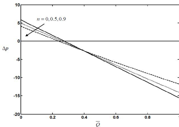
Fig. 10 The variation of the pressure rise \Delta p with \bar{Q} for different values of n with We=0.01 , \beta=0.1 , m=0.2 , Da=0.1 , M=1 and \phi=0.6 .
