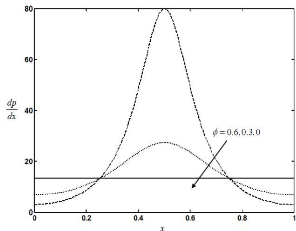
Fig. 8 The variation of the axial pressure gradient \frac{dp}{dx} with \phi for n=0.5 , m=0.2 , M=1 , \beta=0.1 , Da=0.1 , We=0.01 and \bar{Q}=-1 .
