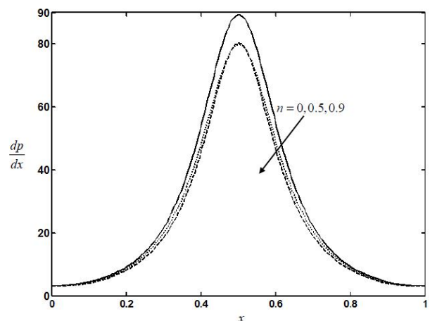
Fig. 3 The variation of the axial pressure gradient \frac{dp}{dx} with n for We = 0.01 , m = 0.2 , M = 1 , \beta = 0.1 , Da = 0.1 , \phi = 0.6 and \bar{Q} = -1 .
