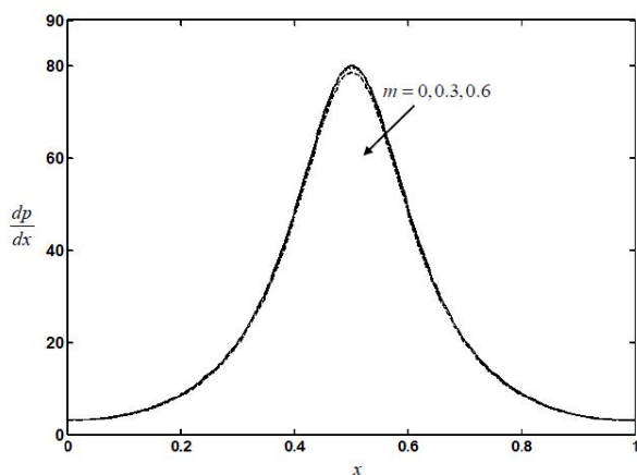
Fig. 6 The variation of the axial pressure gradient
