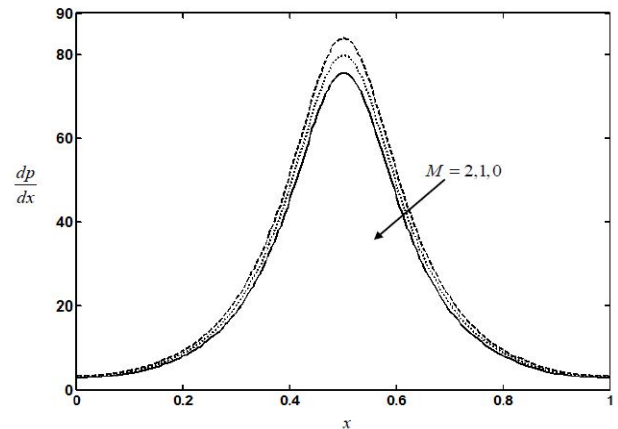
Fig. 7 The variation of the axial pressure gradient \frac{dp}{dx} with M for n=0.5 , m=0.2 , We=0.01 , Da=0.1 , \beta=0.1 , \phi=0.6 and \bar{Q}=-1 .
