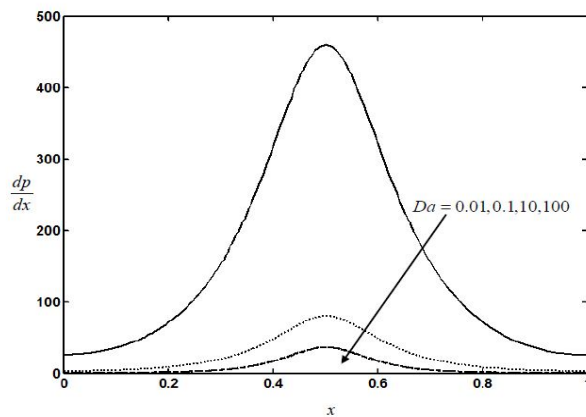
Fig. 5 The variation of the axial pressure gradient \frac{dp}{dx} with Da for n=0.5 , We=0.01 , M=1 , m=0.2 , \beta=0.1 , \phi=0.6 and \bar{Q}=-1 .
