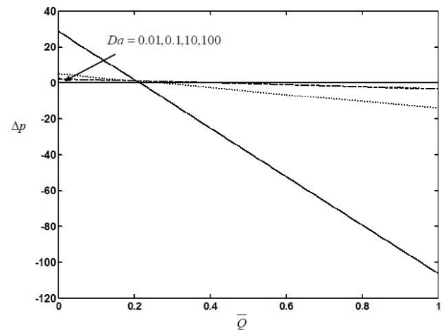
Fig. 12 The variation of the pressure rise \Delta p with \bar{Q} for different values of Da with n=0.5 , m=0.2 , We=0.01 , \beta=0.1 , M=1 and \phi=0.6 .
