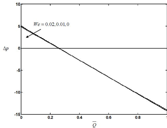
Fig. 9 The variation of the pressure rise \Delta p with \bar{Q} for different values of We with n=0.5 , \beta=0.1 , m=0.2 , Da=0.1 , M=1 and \phi=0.6 .
